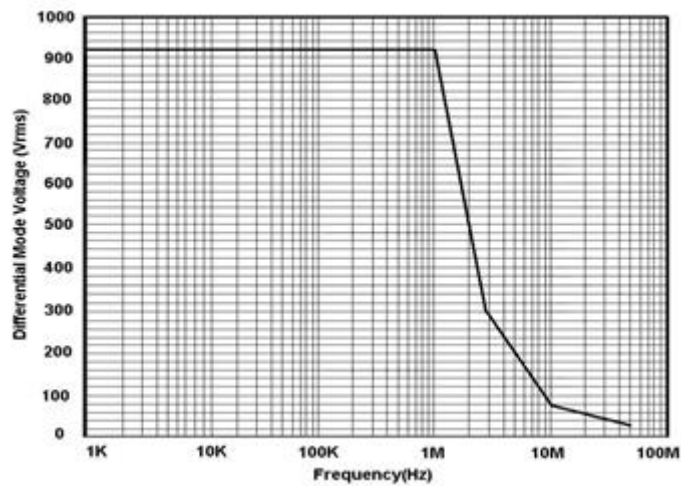
Maximum Differential Voltage VS Frequency Curve
